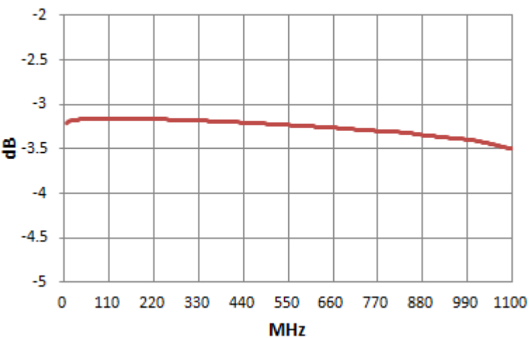
Insertion Loss 1-4
