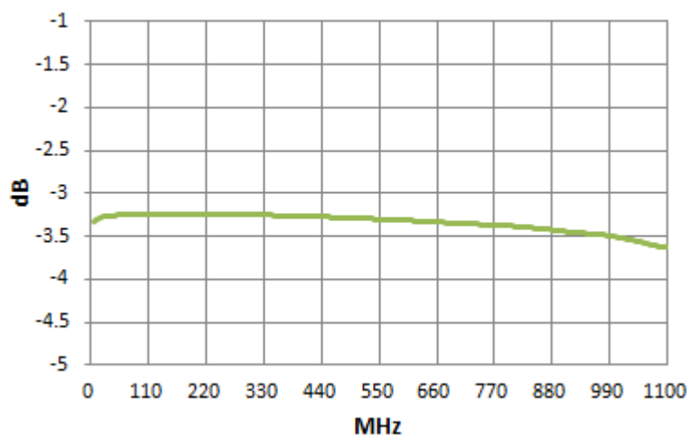
Insertion Loss 1-6
