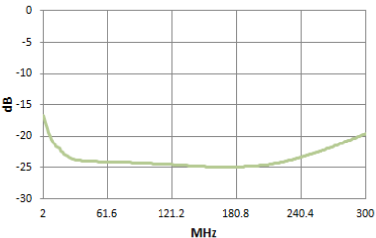
Output Return Loss3
