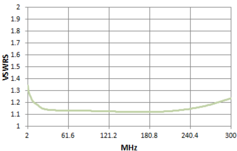
S3-OVSWR
