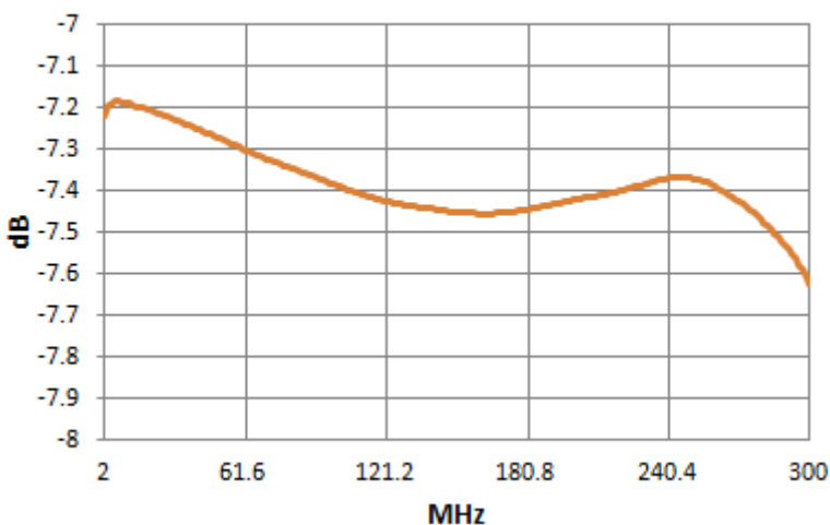
Insertion Loss1-8
