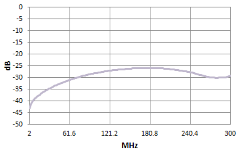
Isolation7-8
