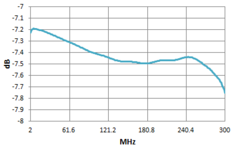
Insertion Loss1-7
