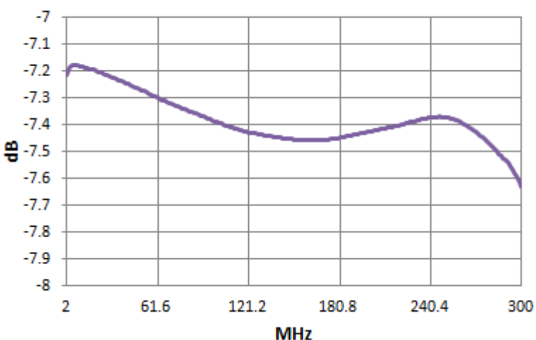
Insertion Loss1-6
