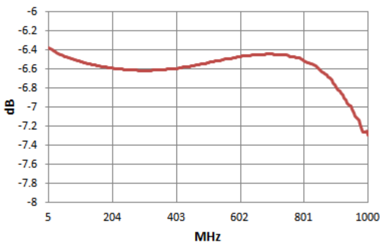
Insertion Loss S-1
