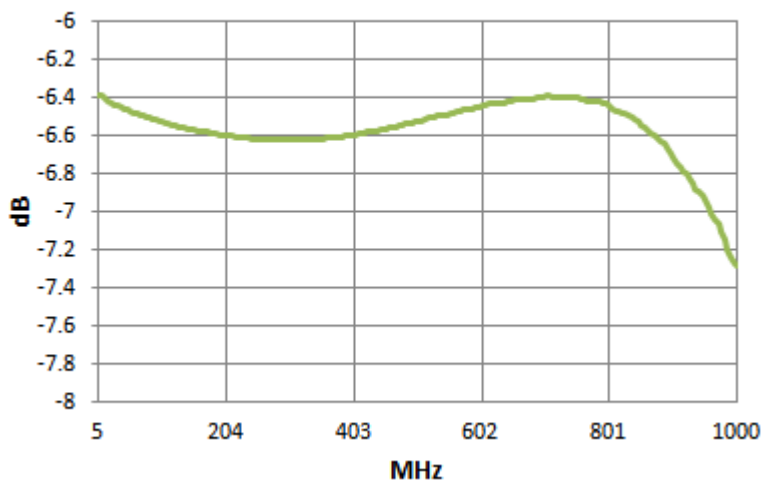
Insertion Loss S-2
