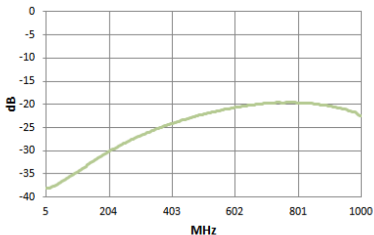
Isolation 2-3
