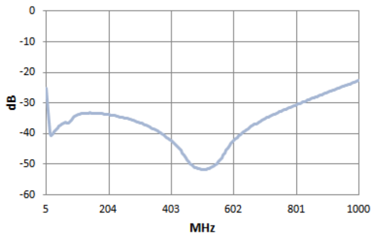
Output3 port3
