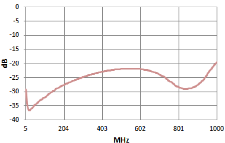
Isolation 1-2
