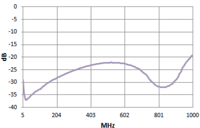
Isolation 3-4
