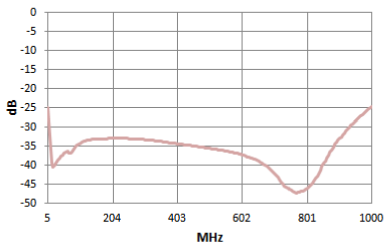
Output4 port4
