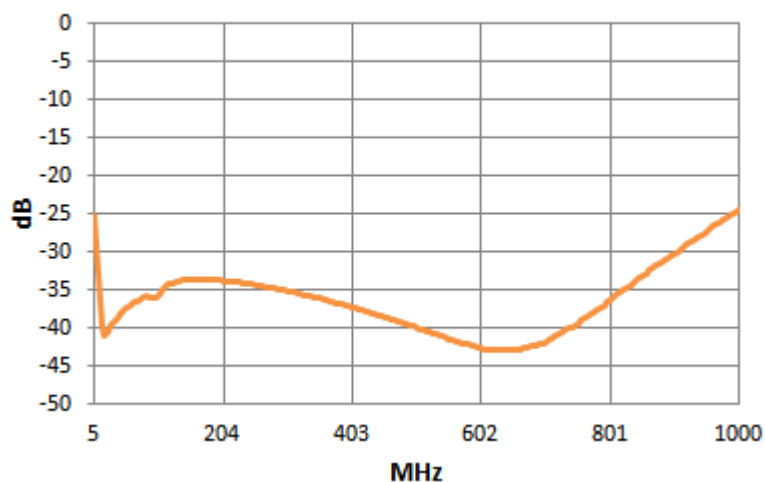
Output2 port2
