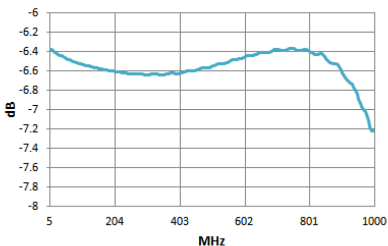
Insertion Loss S-4
